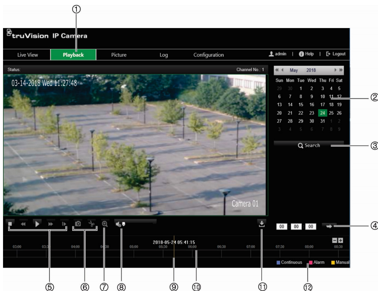
Figure 11: Playback window
