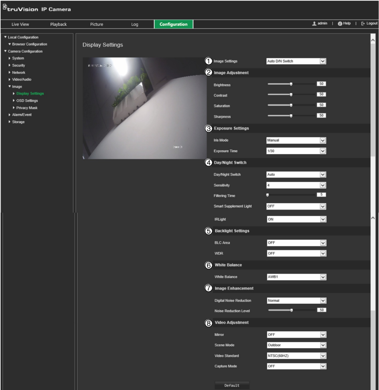
Figure 6: Camera image settings menu – Display Settings tab
