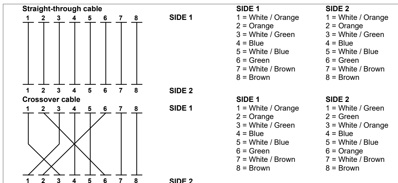
Figure 3: Straight-through and crossover cable
