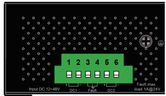
Figure 2: Industrial PoE+ switch upper panel
