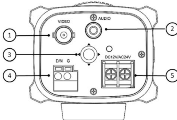
Figure 1: Camera UVC-6130-1-P/N
