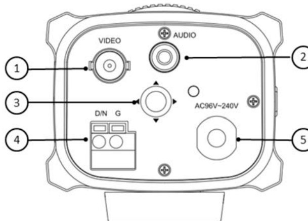
Figure 2: Camera UVC-6130-1-P2
