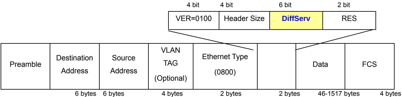
Figure 4-15-4: IPv4 frame format
