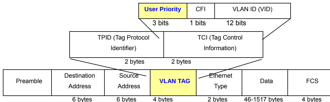
Figure 4-15-1: 802.1p Tag Priority
